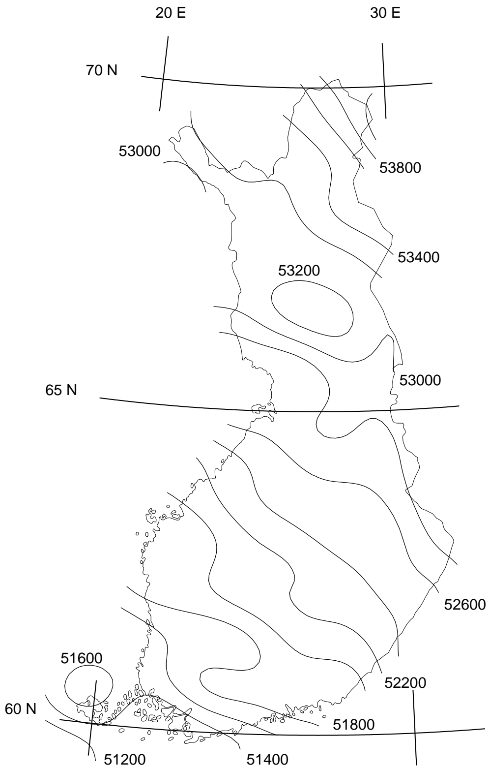
Figure 16: Total intensity F 2007.0 in nT
