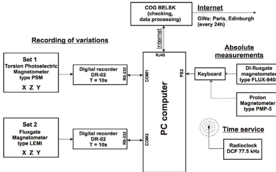
Fig. 7. Block diagram of the magnetic observations system at the Polish Polar Station Hornsund.
